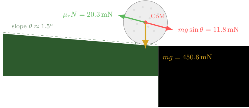
Figure 2: Force diagram of the ball at rest on the lip, all vectors emanating from the center of mass. Gravity acts vertically; its component tangent to the slope drives the ball toward the hole; rolling resistance from the grass canopy opposes the slope force. Slope angle exaggerated for clarity.
