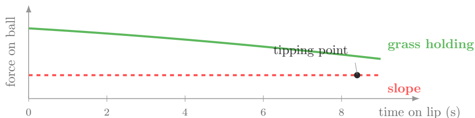
Figure 4: Schematic of the grass giving way. Slope force (red, dashed line) remains constant. The grass’s holding force (green) decreases with time as the blades creep and surface moisture varies. The ball tips when the holding force falls to the slope force. The tipping point is set by the slowly varying factors, not whatever perturbation happens to be around at the time.
