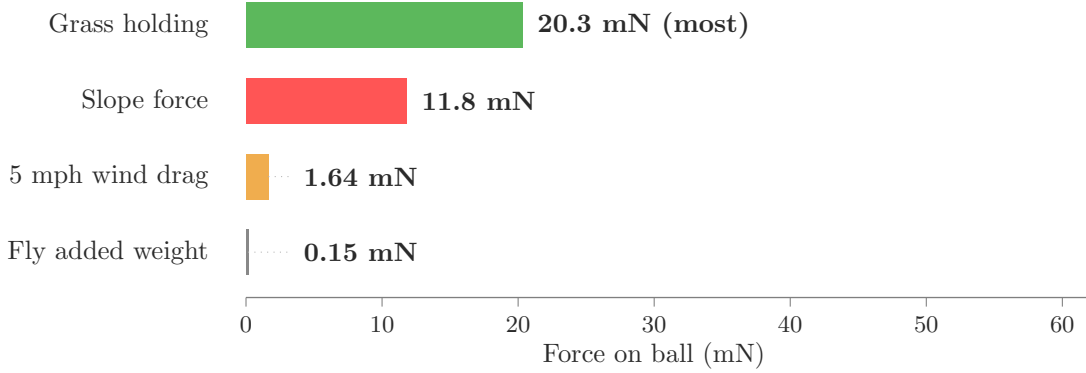
Figure 3: The total force budget, to scale. Green keeps the ball in place. Red is trying to move it. Orange is the wind. Grey is the fly. The fly force is dwarfed by the wind, which is dwarfed by the slope, which the grass holds back with a margin of only 1.7.
